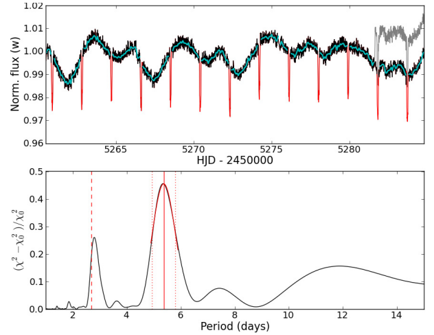
Fig. 2. Top: CoRoT light curve in black with the 13 transits shown in red. All epochs in this paper are given in Heliocentric Julian Date (HJD UTC ; Eastman et al. 2010). The original light curve (shown in gray) contained a discontinuity at HJD -2\,450\,000 = 5281.62 , which was corrected by subtracting 15 mmag from data taken after this date. A linear fit to the light curve has also been used to remove any trend on timescales longer than the duration of the run. The light curve overplotted in blue is binned to one point per orbital period of the CoRoT satellite to make sure that no systematics from the rotation period can come through. Bottom: Lomb-Scargle periodogram of the out-of-transit light curve (black curve in top panel) as a function of relative improvement in \chi^2 compared to a constant flux model. It shows the stellar rotation signature at 5.4 \pm 0.4 days (solid red line), as well as its first harmonic (dashed red line). Also shown are the Gaussian fit used to estimate the uncertainty in the stellar rotation period and the resulting 1- \sigma interval (dotted red lines).
