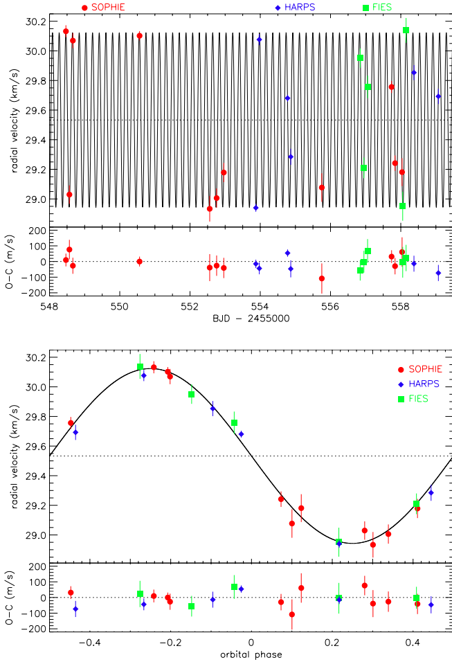
Fig. 4. Upper panel: radial velocity measurements of CoRoT-18 with 1\text{-}\sigma error bars as a function of time together with their Keplerian fit ( top ) and residuals of the fit. The fit is described below in Sect. 4.4. Lower panel: same as above but as a function of the orbital phase. The data are from SOPHIE (red circles), HARPS (blue diamonds), and FIES (green squares).
