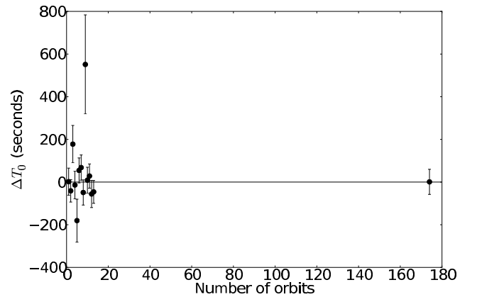
Fig. 9. Transit timing variation \Delta T_0 for each transit of CoRoT-18b. The 13 transits observed with CoRoT (on the left) were obtained about ten months before those observed with Euler (on the right). The 5th and 9th CoRoT transits do cover neither the ingress nor egress and therefore could conduct to erroneous timing measurements.
