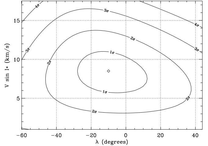
Fig. 12. \chi^2 isocontours for our modeling of the Rossiter-McLaughlin effect as a function of \lambda and v \sin i_* . The diamond shows the lowest- \chi^2 value.
