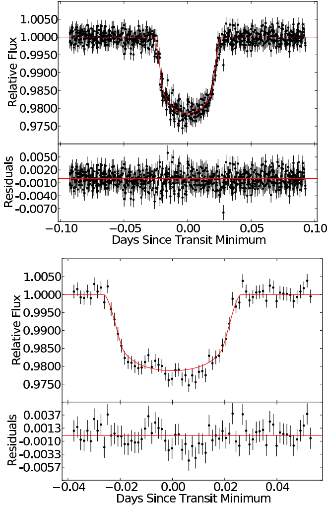
Fig. 3. Phase-folded CoRoT ( top panel ) and Euler ( bottom panel ) transit light curves with the best fit and the residuals. CoRoT data cover 13 transits with a 512-s bin and the Euler data one transit with a \sim 3 -min bin. Both datasets are joint-fitted (see Sect. 4.1).
