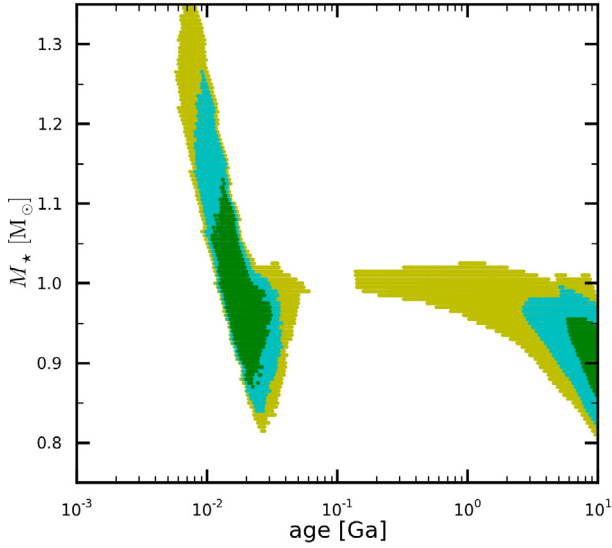
Fig. 10. Constraints obtained from stellar evolution models for the age and mass of CoRoT-18. The colored circles correspond to constraints derived from stellar evolution models matching the stellar density and effective temperature within a certain number of standard deviations: less than 1\sigma (green), 2\sigma (blue), or 3\sigma (yellow).
