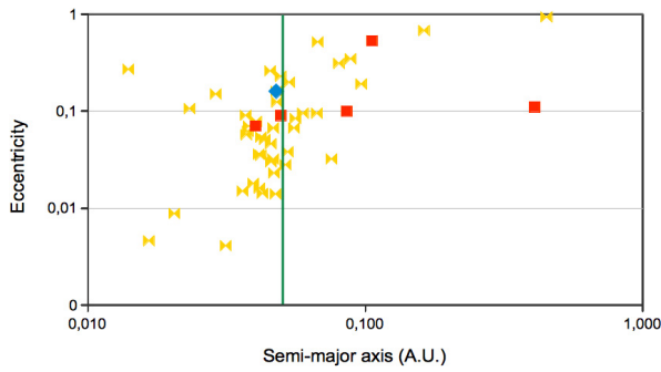
Fig. 12. Diagram of eccentricity vs. semi-major axis of the different transiting planets that have no-zero eccentricity. We display with different symbols the ones discovered by CoRoT (red squares), by other experiments (yellow bowties), and by CoRoT-23b (blue diamond). The vertical line marks an arbitrary frontier between hot and warm Jupiters.
