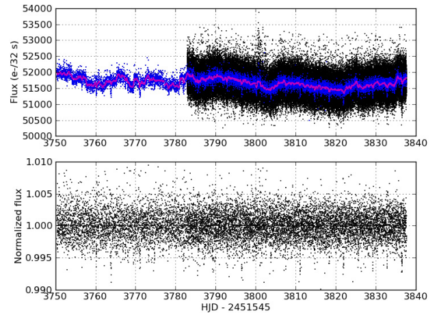
Fig. 1. CoRoT LC of the target CoRoT-23. The apparent change of regime at CoRoT JD 3783 corresponds to the change in the sampling period from 512 s to 32 s. Upper panel: raw data (in black), at a unique sampling period of 512 s (blue) and after a median-smoothing on 10 h (purple). Lower panel: LC after applying a detrending filter.
